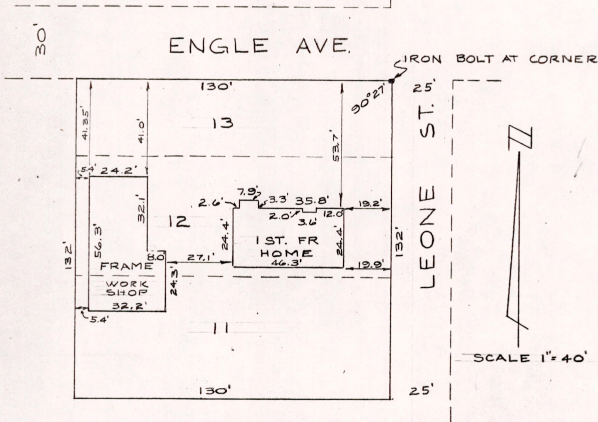
SURVEY OF LOTS 11-12-13, BLOCK 20 2ND ADD. TO THE DELLWOOD
